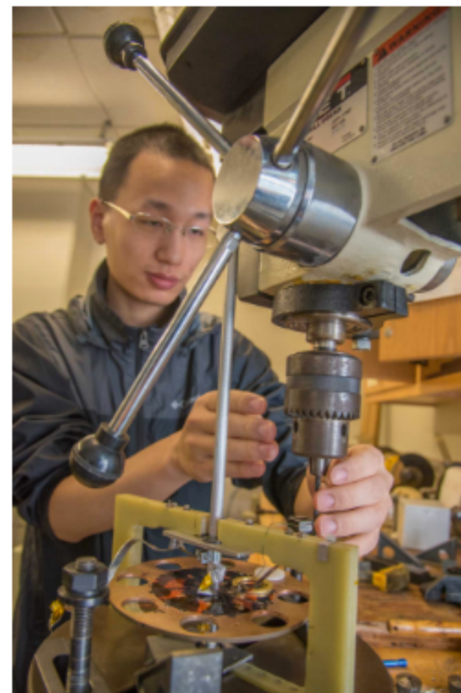
Simon Liu '17 played a major role in developing and testing this unique filter wheel that holds up to eight different cosmic dust samples.
