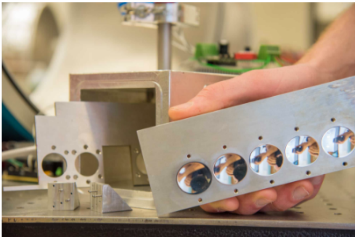
A physics student displays an ellipsoidal mirror, which is installed inside the spectrometer.
