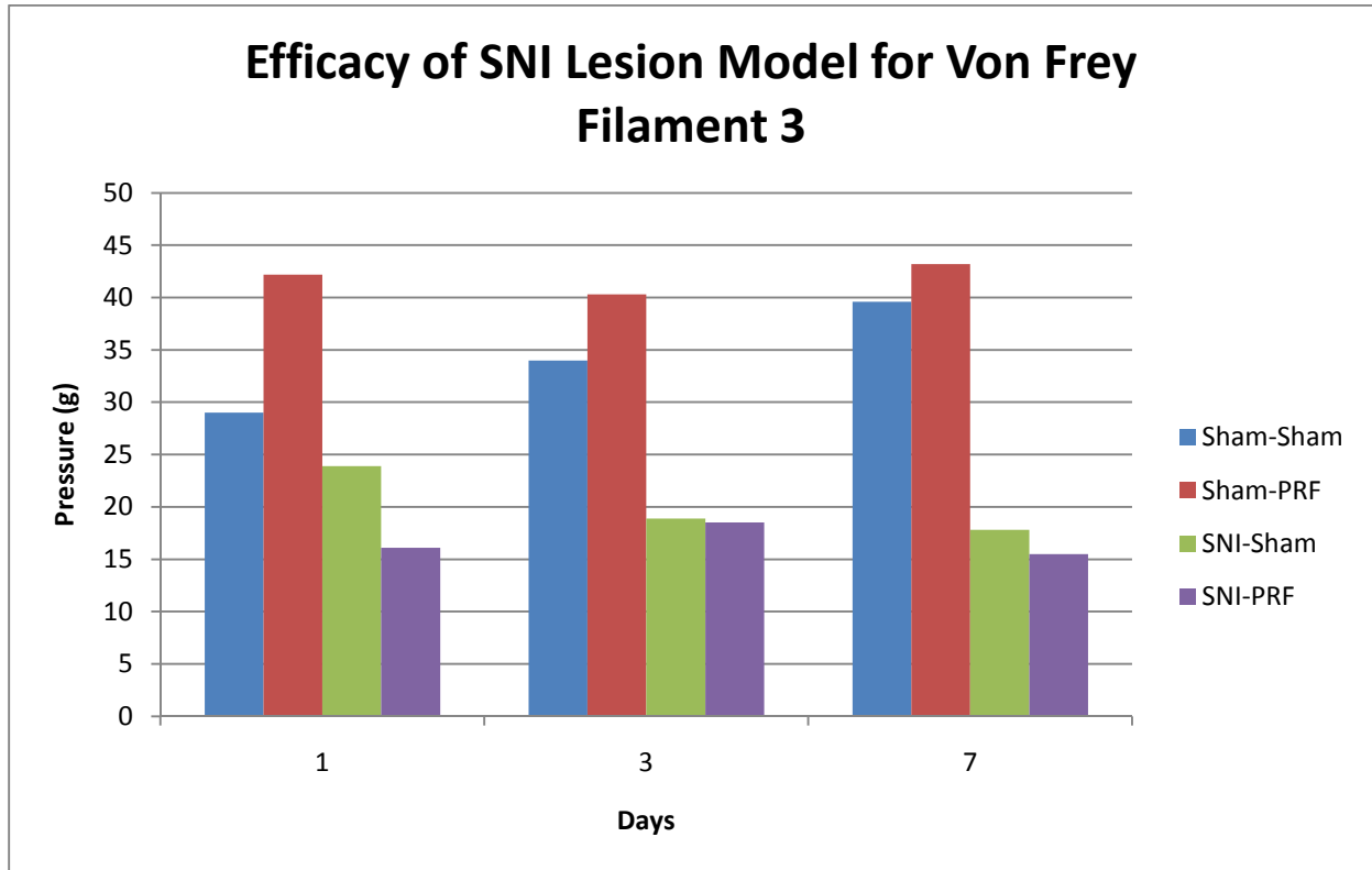
Figure 4. There was a significant difference between the SNI lesion model groups and the groups that did not receive the SNI lesion for Filament 3. This indicates that the SNI lesion model effectively put the rats into a state of chronic hypersensitivity.
